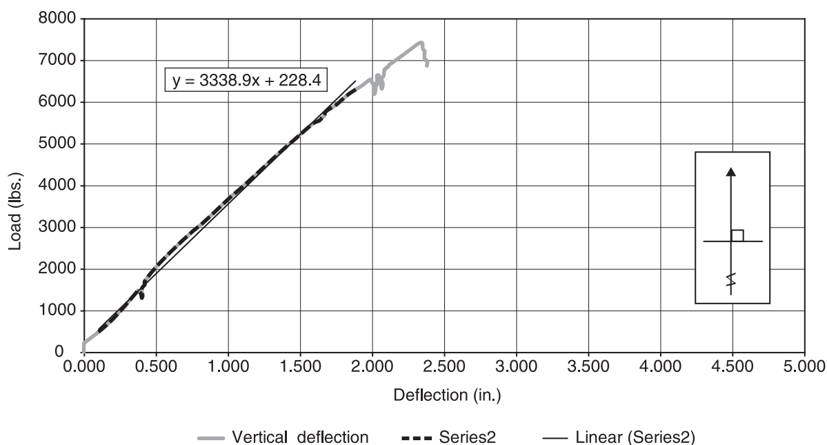
Figure 7-6. Typical response for an axially loaded anchor.
